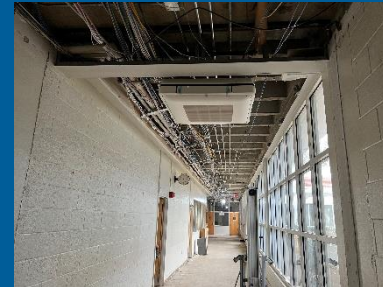
Installation of VRF cassette unit in front hallway
